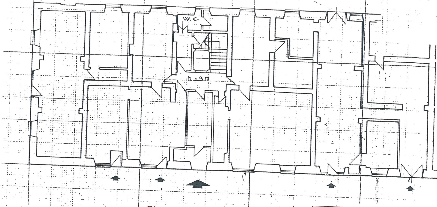
PIANO TERRA
